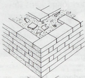
Metselverbanden in baksteen
